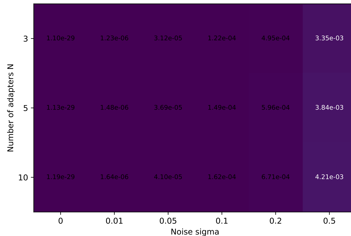
Rank r = 32
