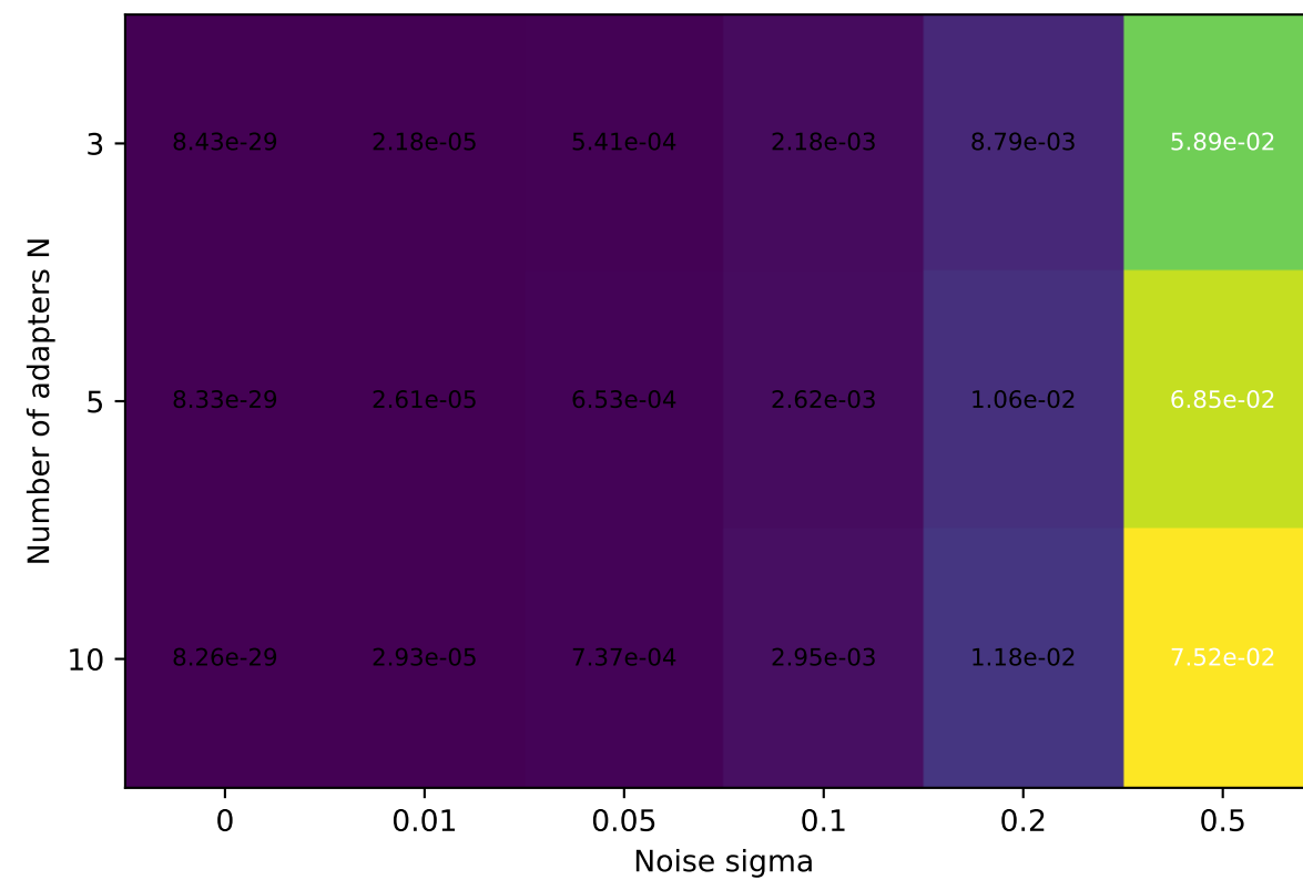
Rank r = 32
