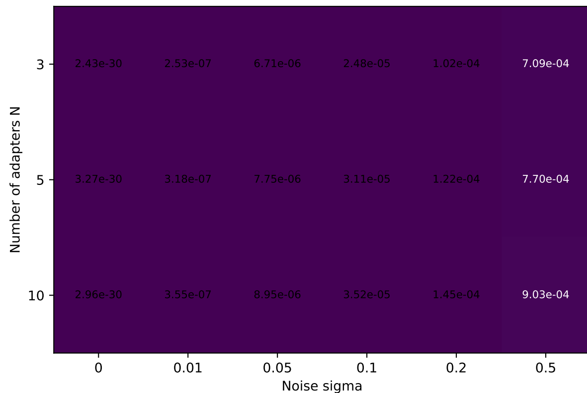
Rank r = 16
