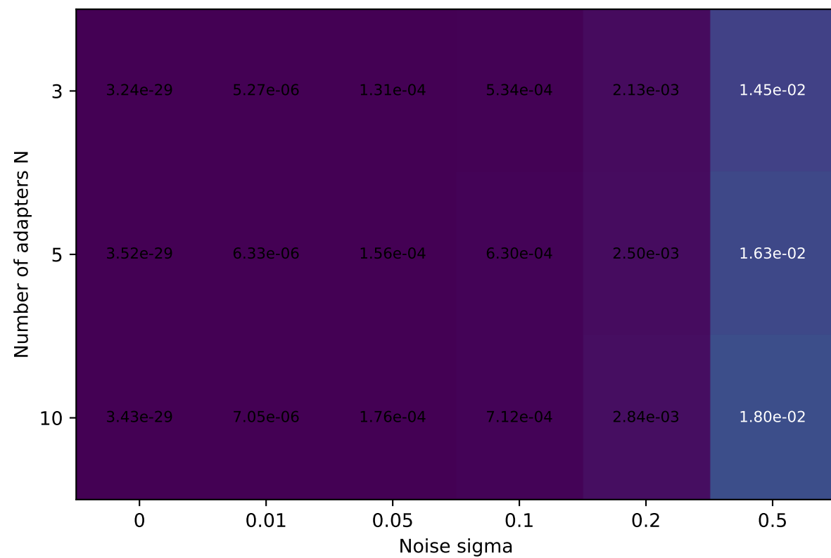
Rank r = 16
